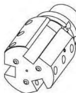
Axial toolholder 25x25 mm 142-21605 (left) 142-11605 (right)
