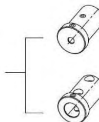
Boring bar holder Ø40 mm 145-21605
