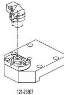
Face and O.D. cutting holder HSK 40 A+C
