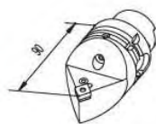
H63APCMNR12-90
