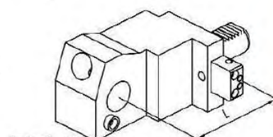
115-54143 (L=100) 115-54145 (L=120)
