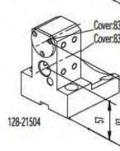
Combi toolholder for boring bar and insertdrill with internal coolant Ø20 mm
