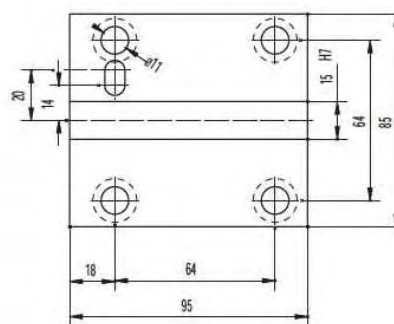
Boring bar sleeve
