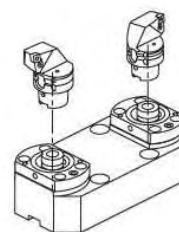
Face and O.D. cutting holder HSK 40 A+C
